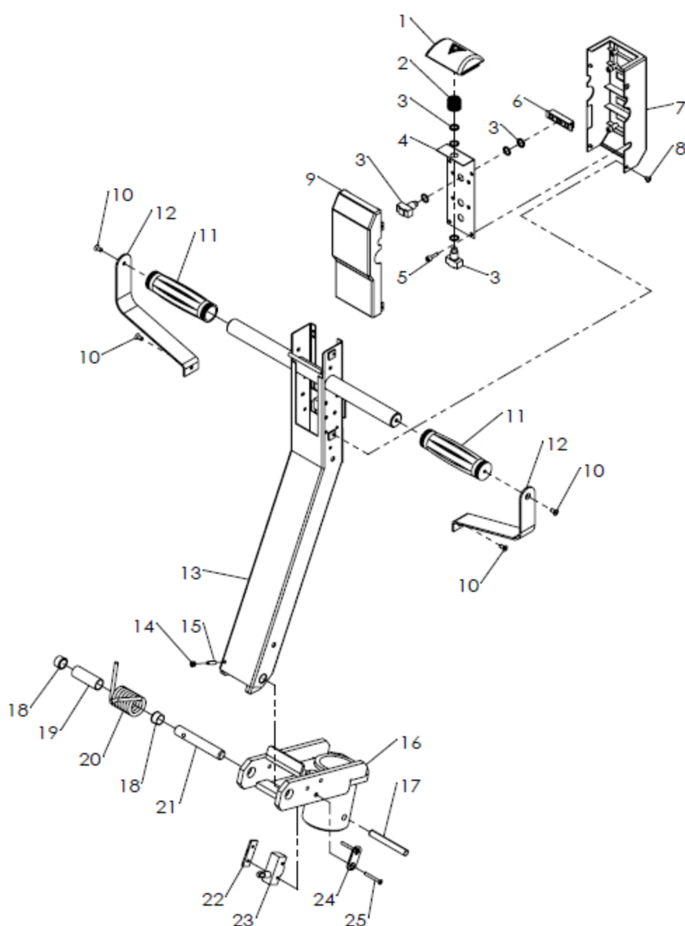
HANDLE1
