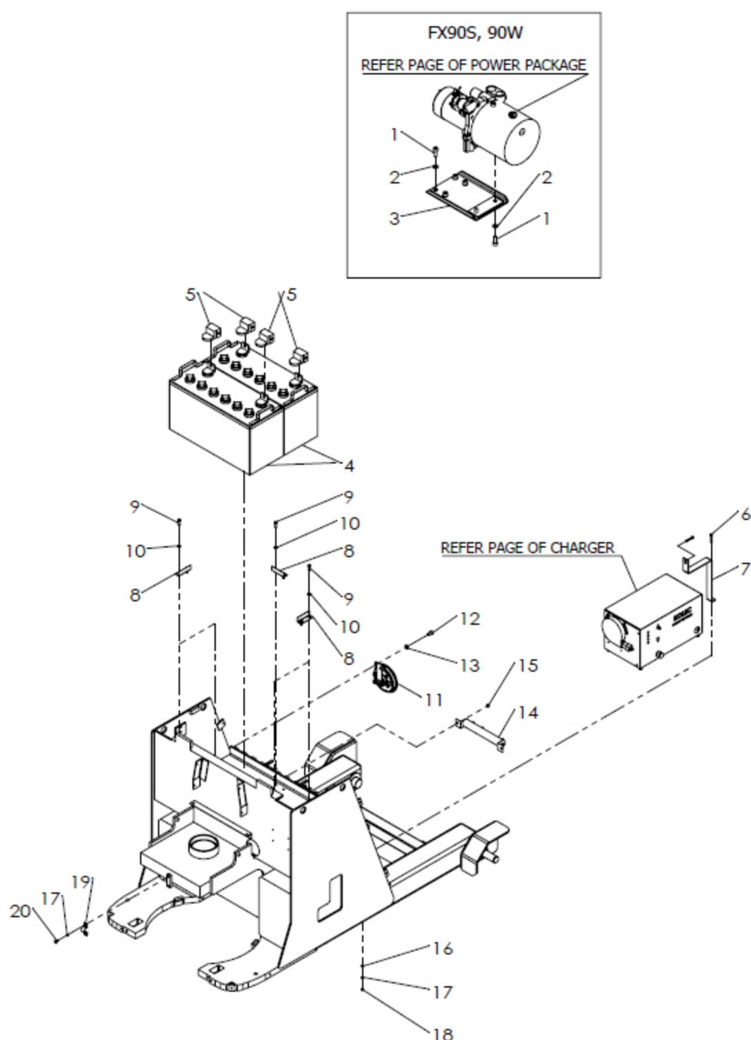
FRAME 1
